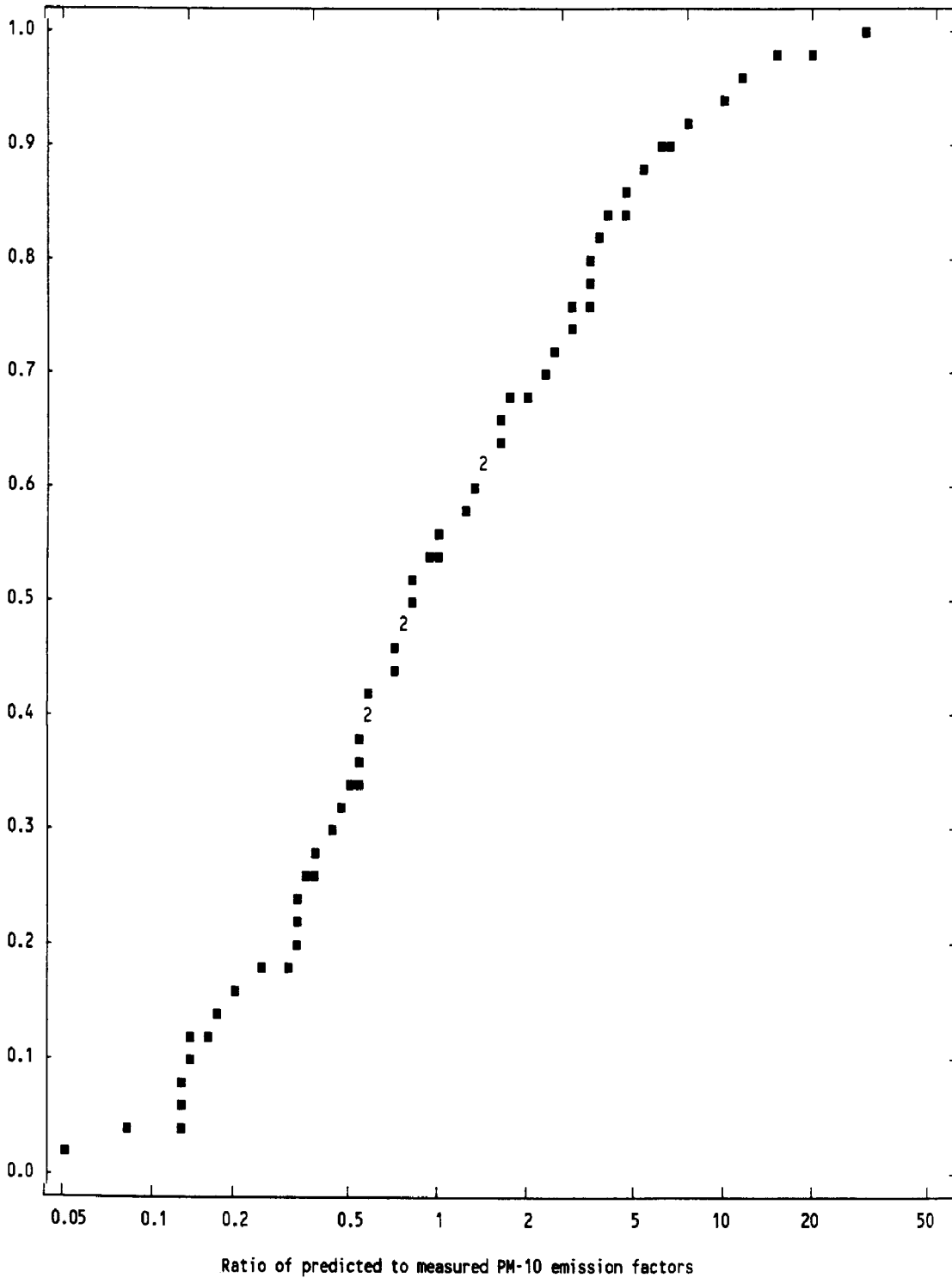
Figure 4-4. Cumulative frequency distribution obtained during cross-validation study.
